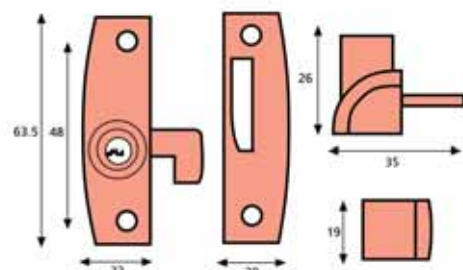
Flush Pivot Lock
