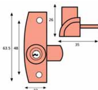
Metal Window Lock
