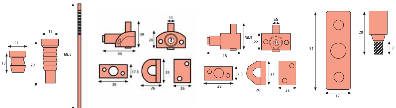
Window Bolt - Key Cut
